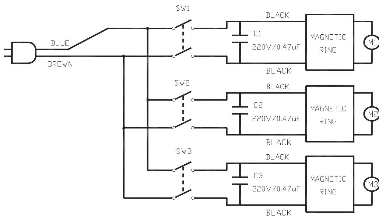
Wiring Diagramme for LSU375 & LSU395 (Figure 9)
