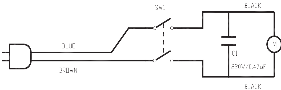
Wiring diagramme for LSU135 & LSU155(Figure7)
