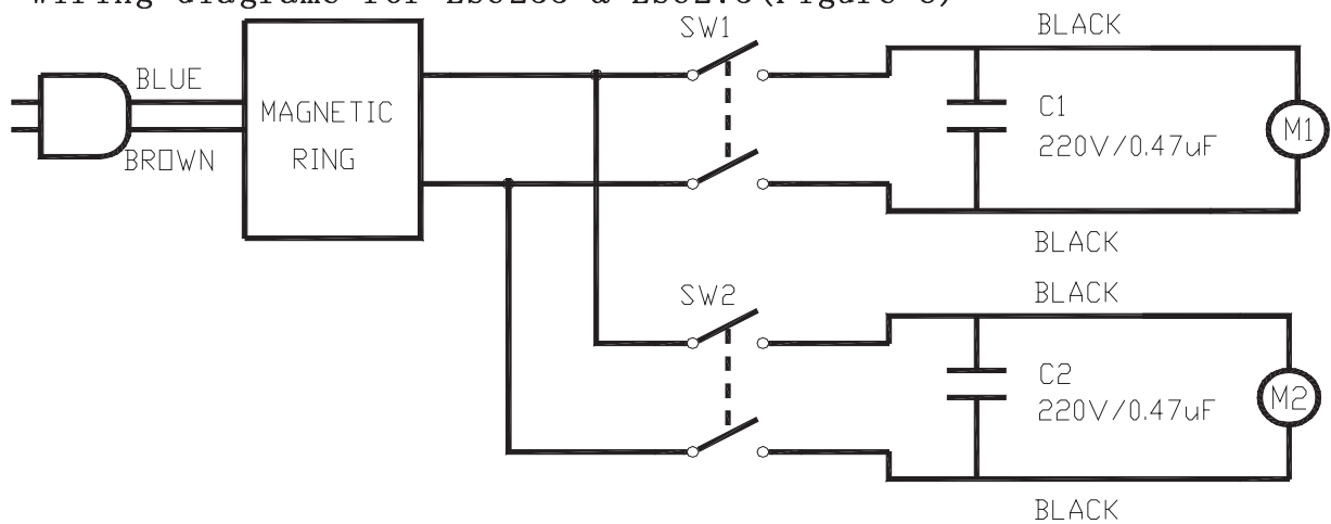
Wiring diagramme for LSU255 & LSU275(Figure 8)
